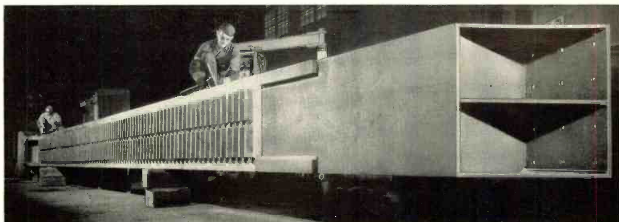
World's Biggest Crowd. On power shovels, a "crowd" is the arm which moves the dipper and dipper-stick forward and back. It coordinates closely with the lift motion of the dipper, and is a key part in the operation of the shovel which must withstand extremes of stress at any temperature. This is a picture of the biggest crowd ever built, now installed on the biggest power shovel in the world. It's made from USS "T-1" Steel, the remarkable new constructional alloy steel developed by United States Steel. An exceptionally strong and tough steel, it is noted for its welding characteristics. "USS" and "T-1" are registered trademarks.
