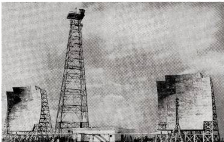
THESE TWO 60 sq. ft. reflectors at Florida City, Fla., make it possible for AT&T to bounce tv signals off the troposphere and furnish live programs between the U. S. and Cuba. The system, to become operative by Sept. 12, uses the scatter mode of radio transmission.
